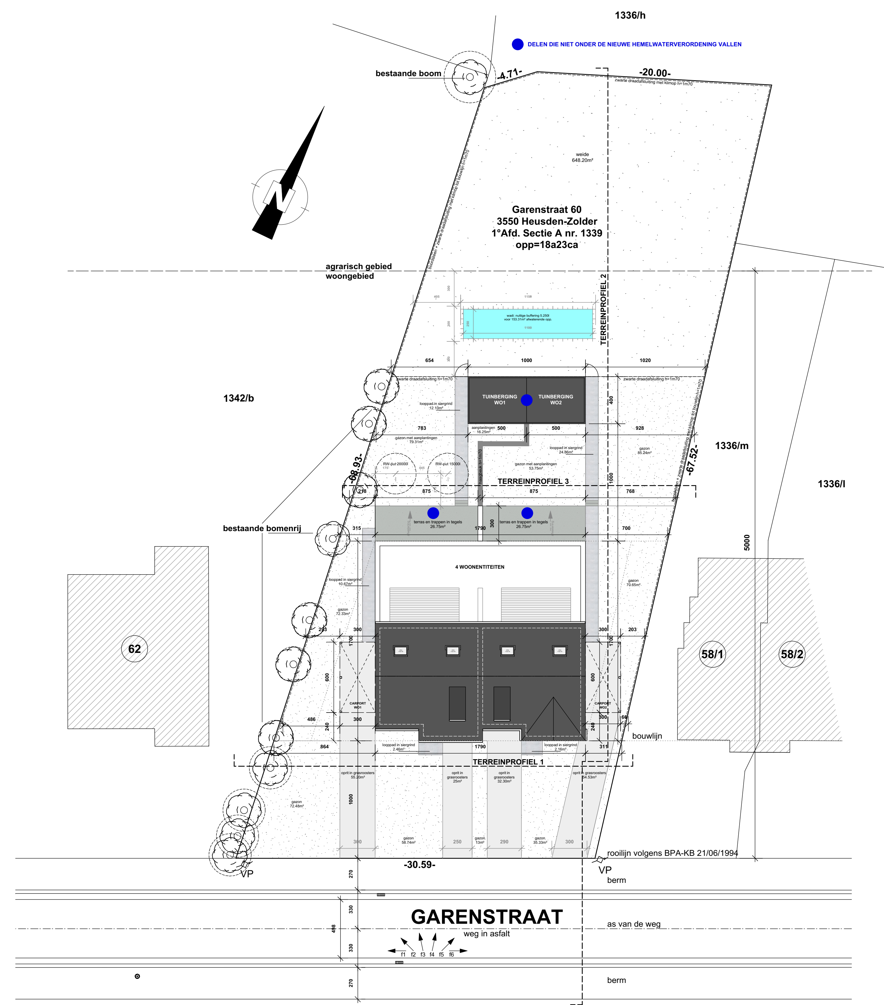
INPLANTING-BEPLANTINSPLAN
