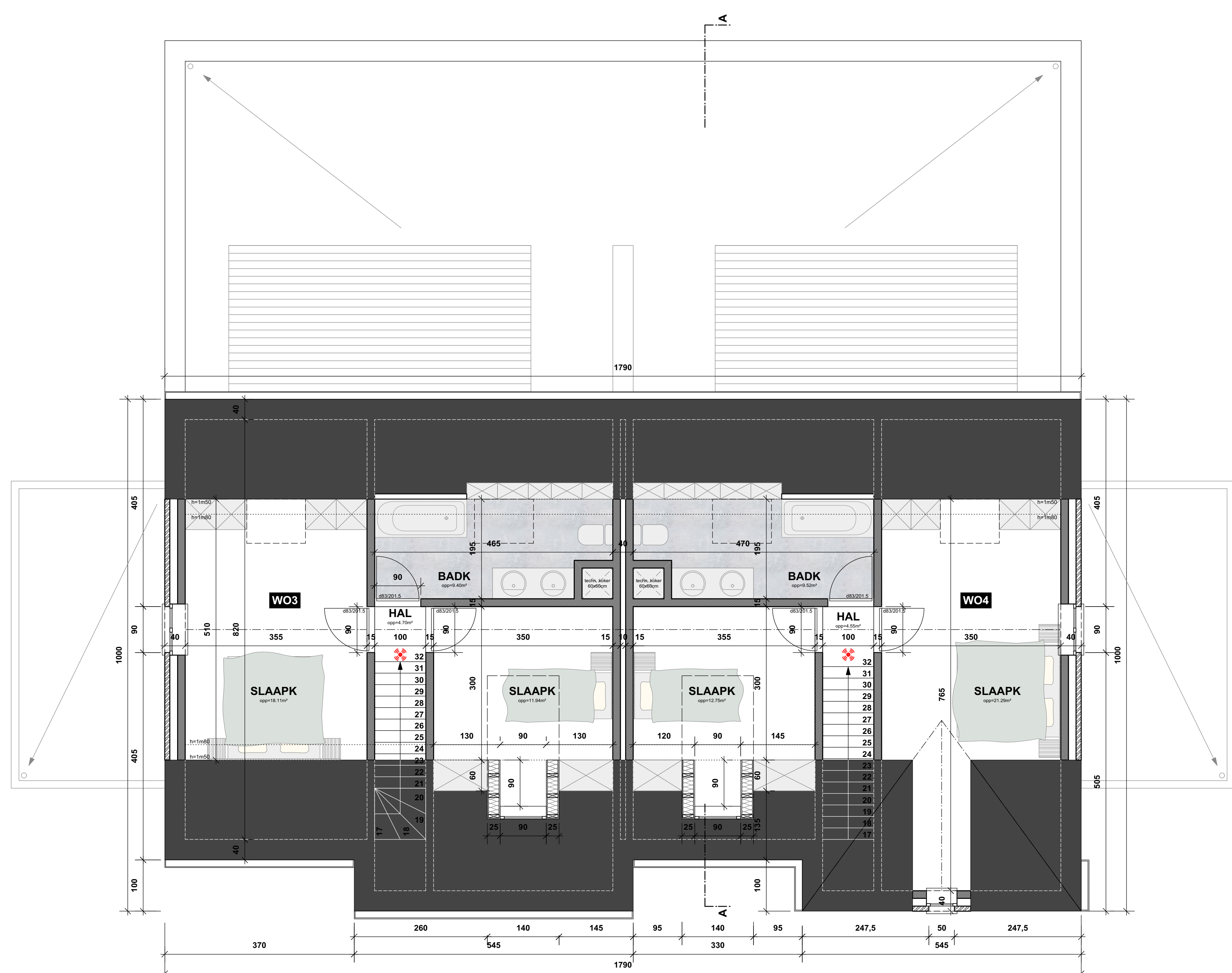
ZOLDERPLAN nivo +5.80
