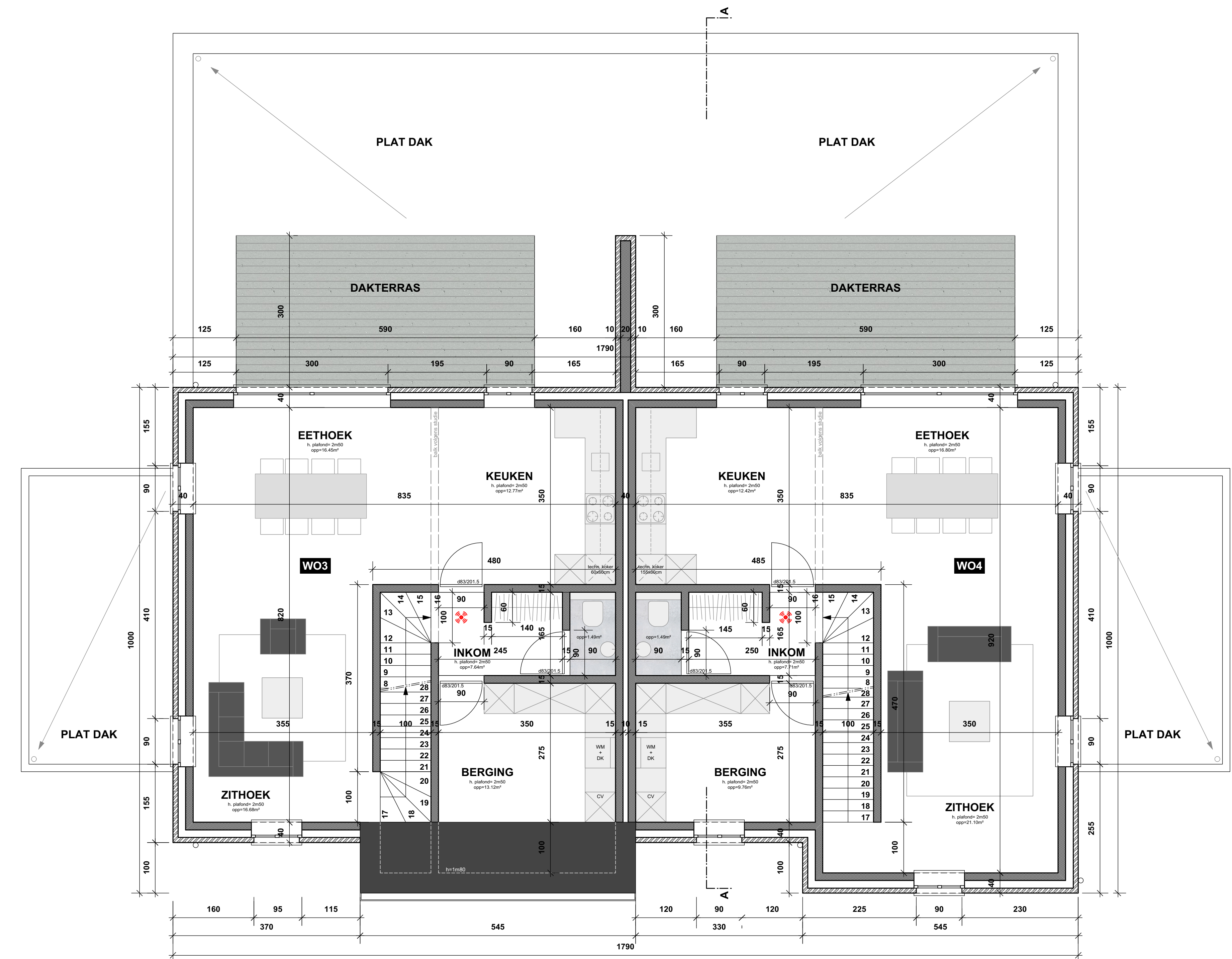
VERDIEPING nivo +2.90
